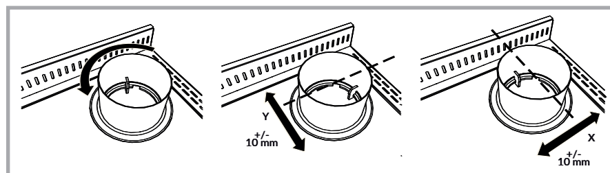
Picture 8 - Tolerance for flue outlet on the top and back. The tolerance depends on the orientation of the connector.
