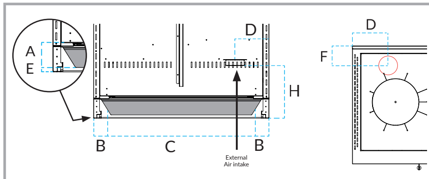
Picture 12 - Rear sight of the plinth of the wood fired cooker and specifies for the connection with the air intake.
