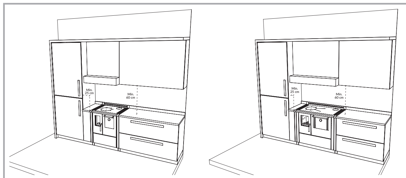
Picture 2 - Minimum safety distances when using suited spacers for the installation into furniture in presence of inflammable materials.
