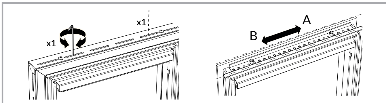
Picture 20 - Auxiliary air adjustment for glass cleaning: the plate is open at the position indicated with the letter A, while it is closed at the position indicated with the letter B.
